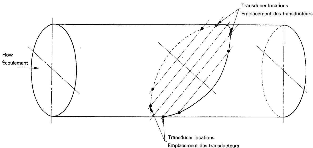
Figure 28 — Arrangement of transducers in a four-path diagonal-beam meter
