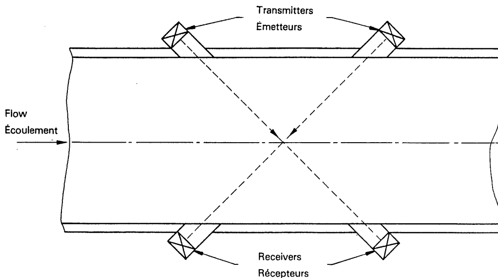
Figure 27 — Principle of operation of the multi-path diagonal-beam meter
