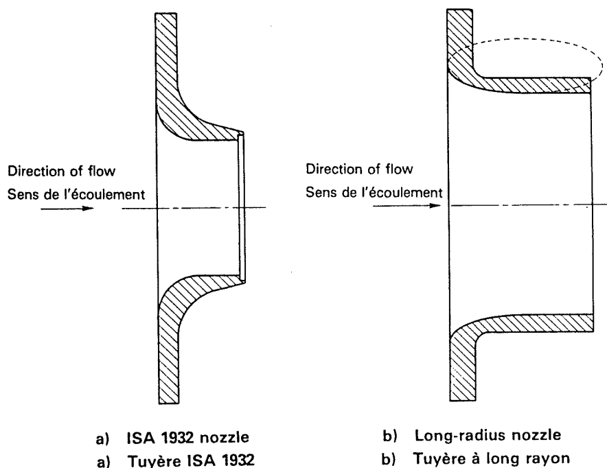
Figure 5 — Nozzles
