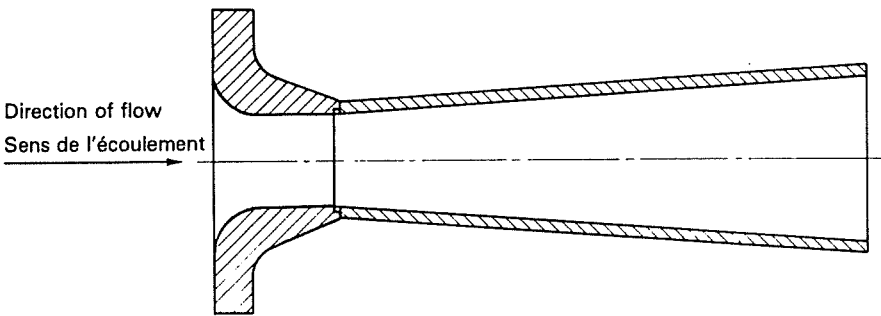
Figure 9 — Cylindrical throat Venturi nozzle Figure 9 — Venturi-tuyère à col cylindrique
