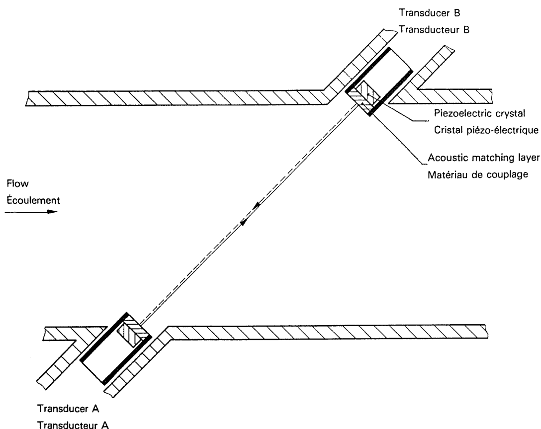
Figure 26 — Principle of operation of the single-path diagonal-beam meter
