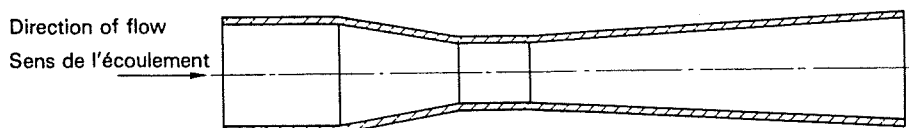
Figure 6 — Classical Venturi tube
