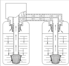
双罐串联系统 Duplex Tanks Work in Series
