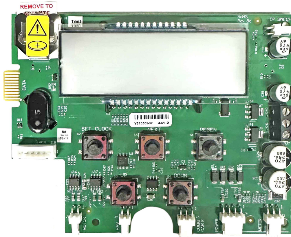
WS1 - WS2QC CI Circuit Board Order Number: V3108CI-07BOARD
